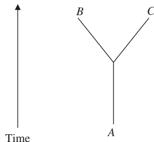
Figure 7.1 A Feynman diagram for the decay process A \rightarrow B + C . Time flows from the bottom of the diagram to the top.
