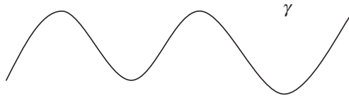
Figure 8.1 A schematic representation of a photon that we will use in a Feynman diagram for QED processes is a wavy line. We can include a \gamma for clarity if desired.
